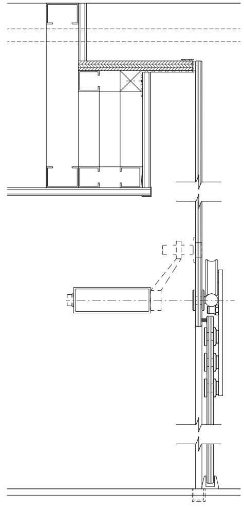
Plan & Section detail at glass TV room enclosure
