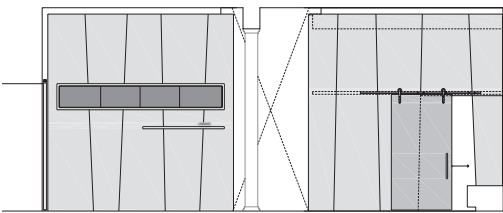
Kitchen sideboard and TV room elevation
