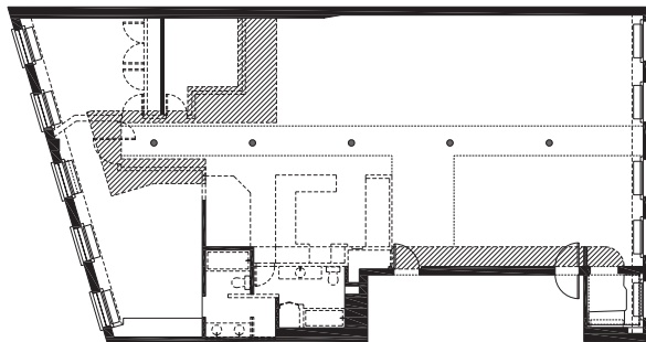
Exiting conditions survey and demolition plan
